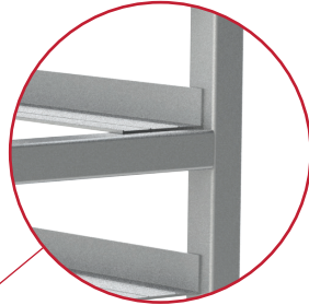
HD Uprights & Cross Braces All welded 1-1/4" square tubular frame with 1" cross braces, all rounded-edges
